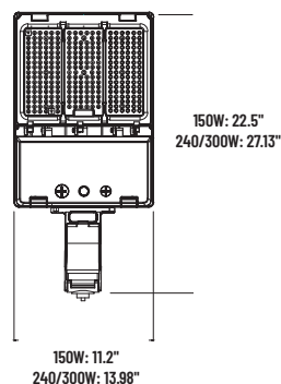
Round/Square Pole Mount
