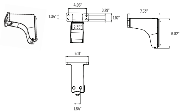
Round/Square Pole Mount
