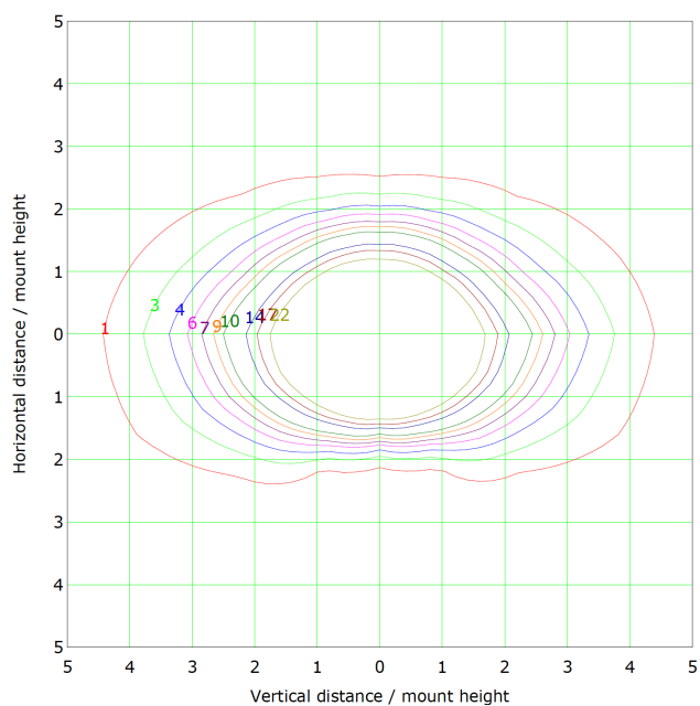
IsoLux Plot
