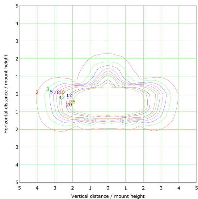
IsoLux Plot
