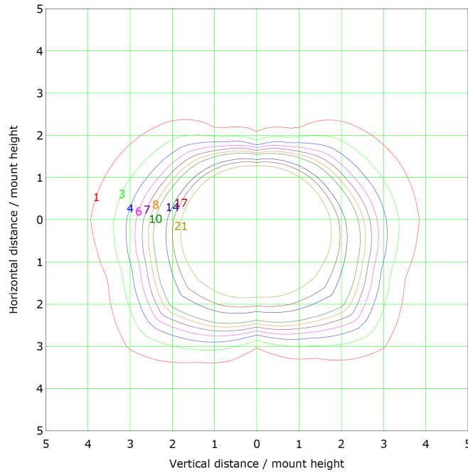
IsoLux Plot
