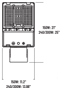
Trunnion Mount
