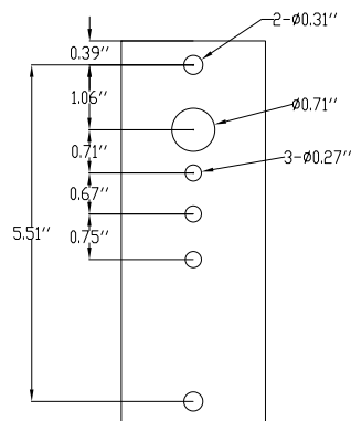
Pole Drilling
