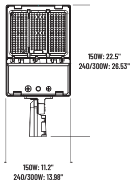
Slipfitter Mount
