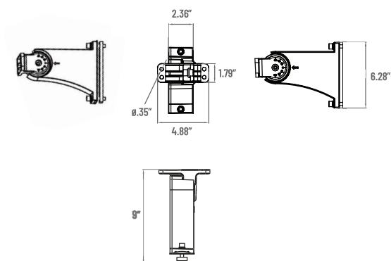
Adjustable Round/Square Pole Mount
