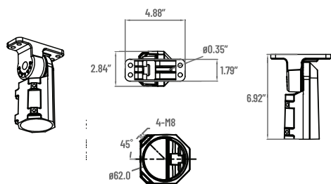
Slipfitter Mount
