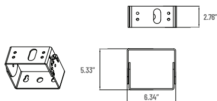
Trunnion Mount
