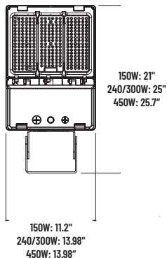
Trunnion Mount
