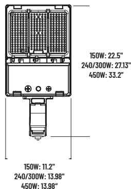
Round/Square Pole Mount
